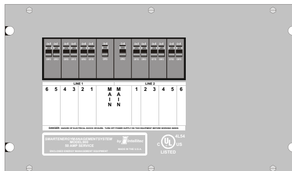
50 Amp EMS Distribution Panel P/N 00-00683-000
